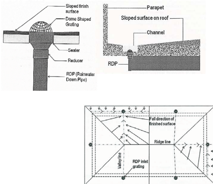
Figure 6: Configurations of gutters and rainwater downpipes on roofs (image source: Rainwater harvesting in buildings (unpublished manuscript) by Syed Azizul Haque, used with permission)
