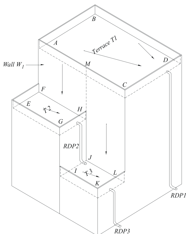
Figure 4: Catchment area of flat roof and surface wall. (Haq, 2006)
