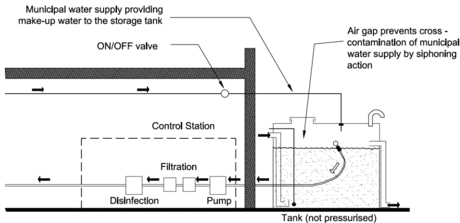
Figure 11: Make-up supply to main tank with air-gap protection (Image source: Novak et al 2014)
